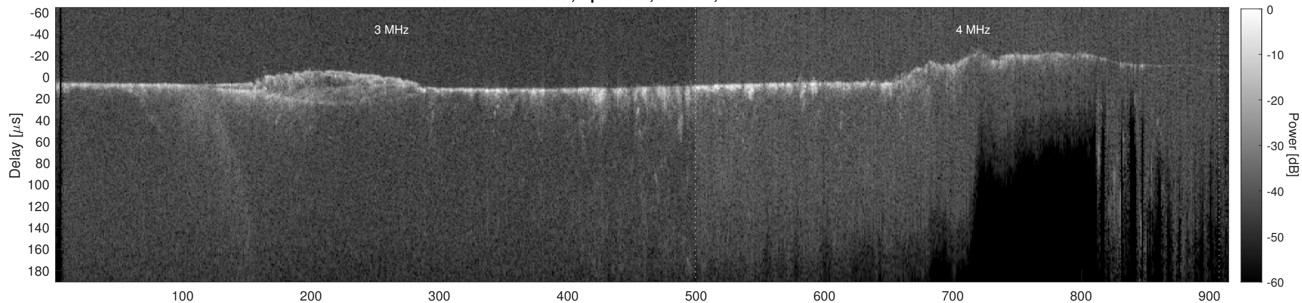
Orbit 11696, Cluttergram
