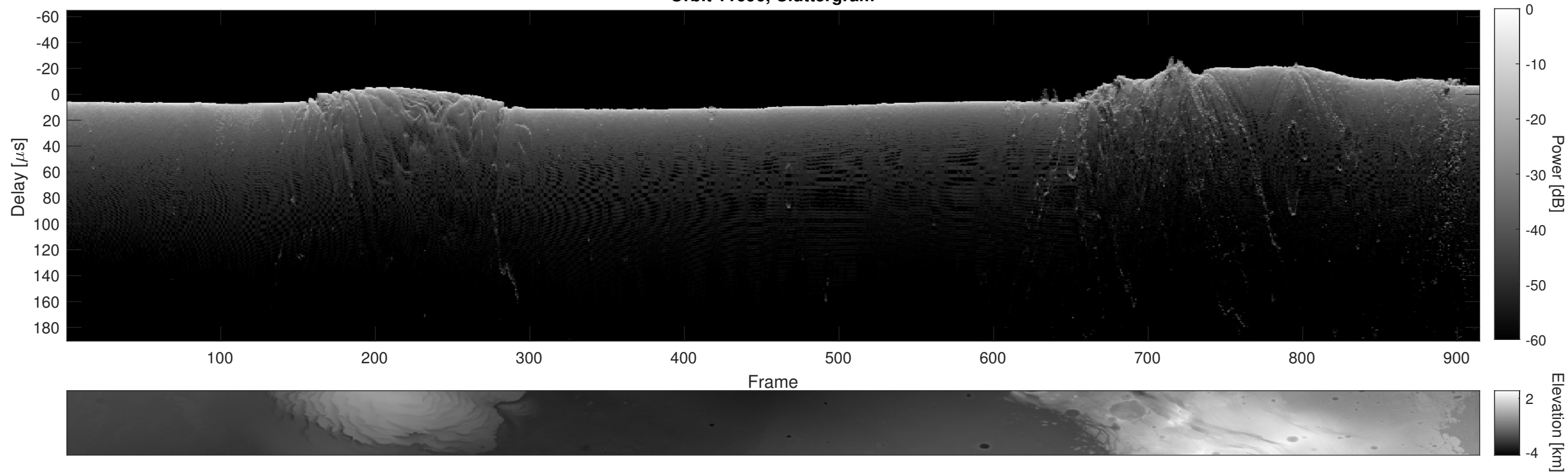
Orbit 11696, Cluttergram
