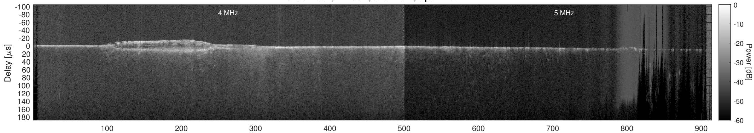
Orbit 11697, Cluttergram
