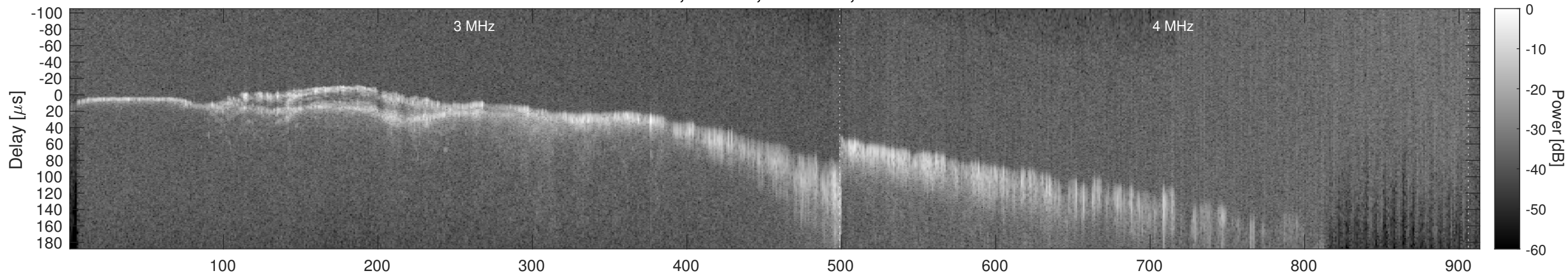
Orbit 11697, Window, Channel 2, Chapman
