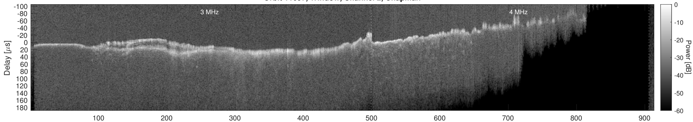
Orbit 11697, Window, Channel 2, Optimized
