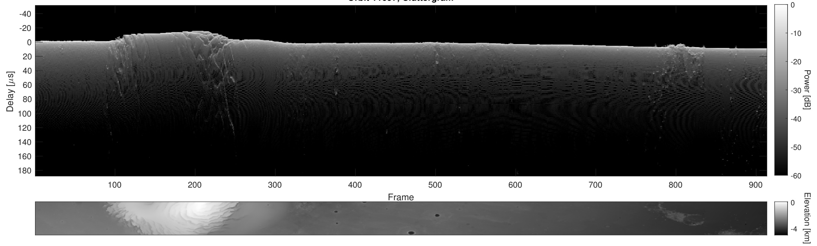
Orbit 11697, Cluttergram
