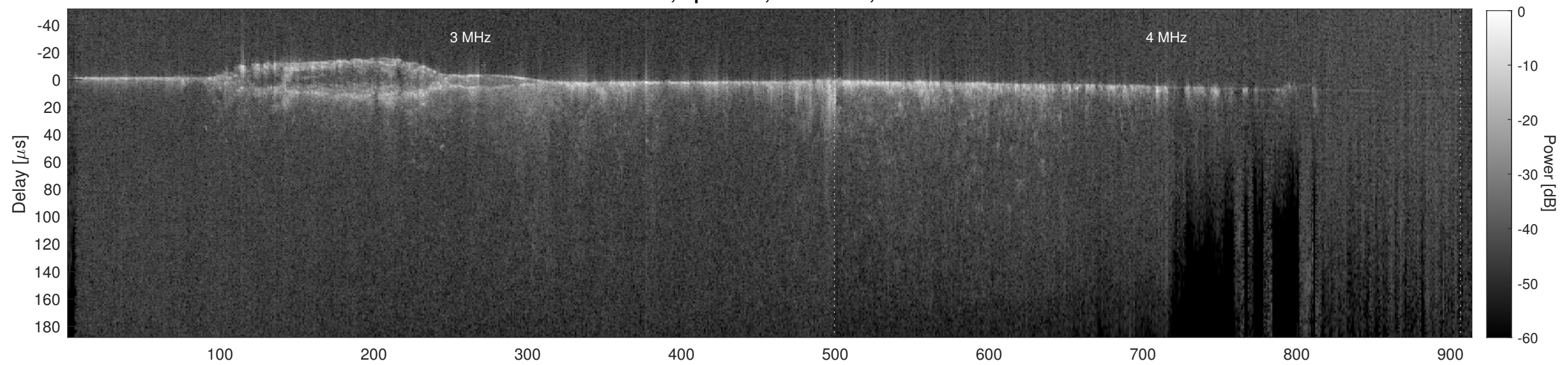
Orbit 11697, Cluttergram
