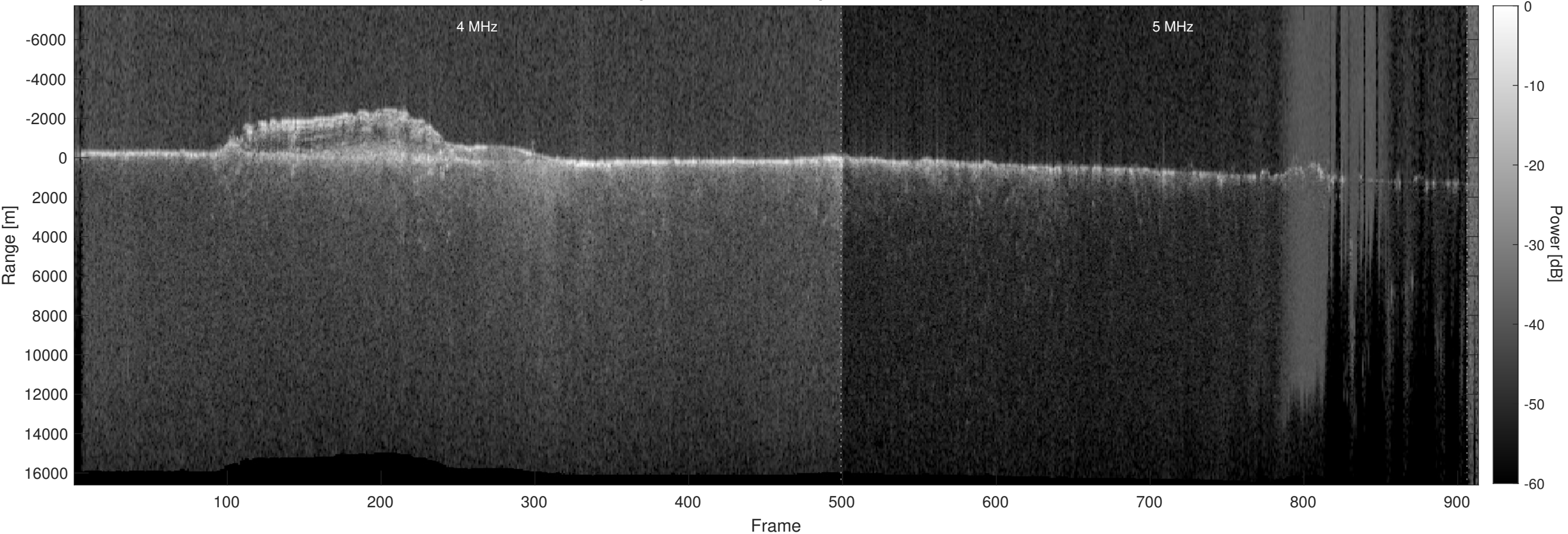
Orbit 11697, Optimized, Window, Depth-Corrected, Channel 2
