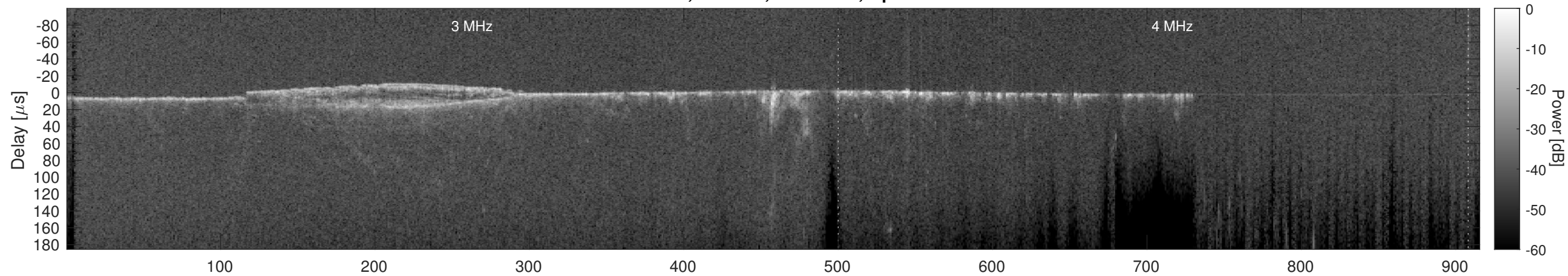
Orbit 11698, Cluttergram
