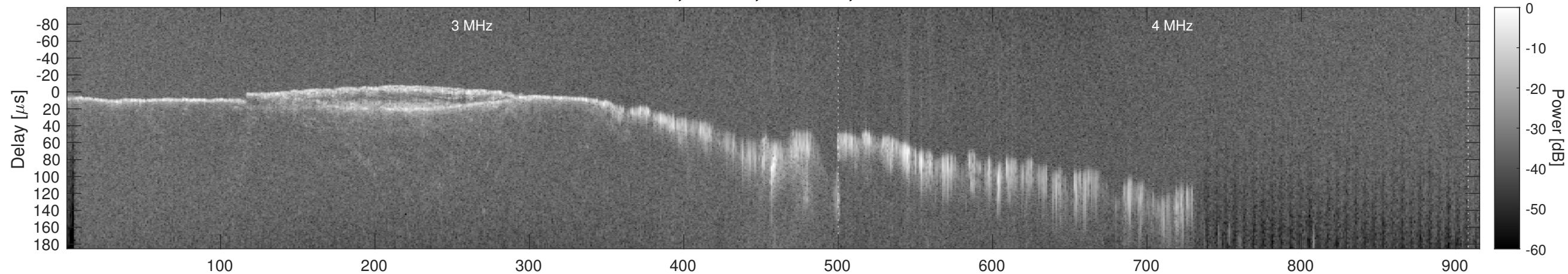
Orbit 11698, Window, Channel 2, Chapman
