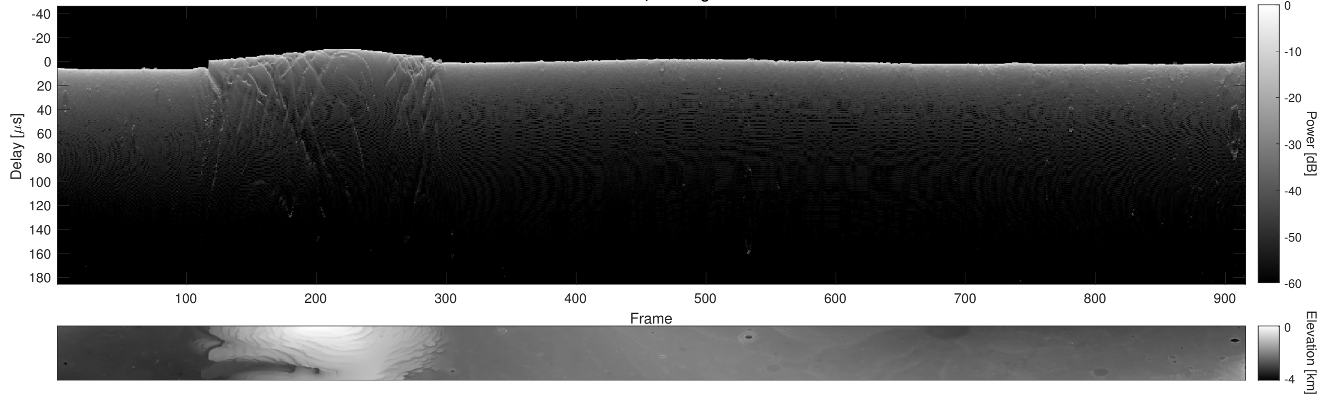
Orbit 11698, Cluttergram
