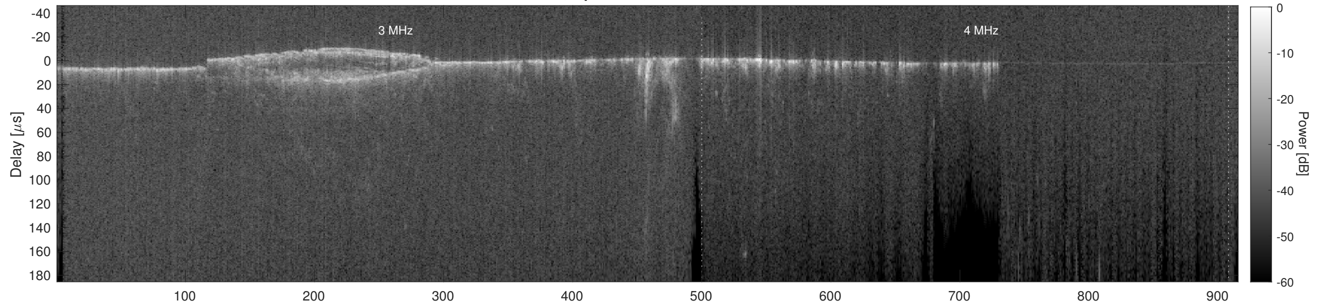
Orbit 11698, Cluttergram
