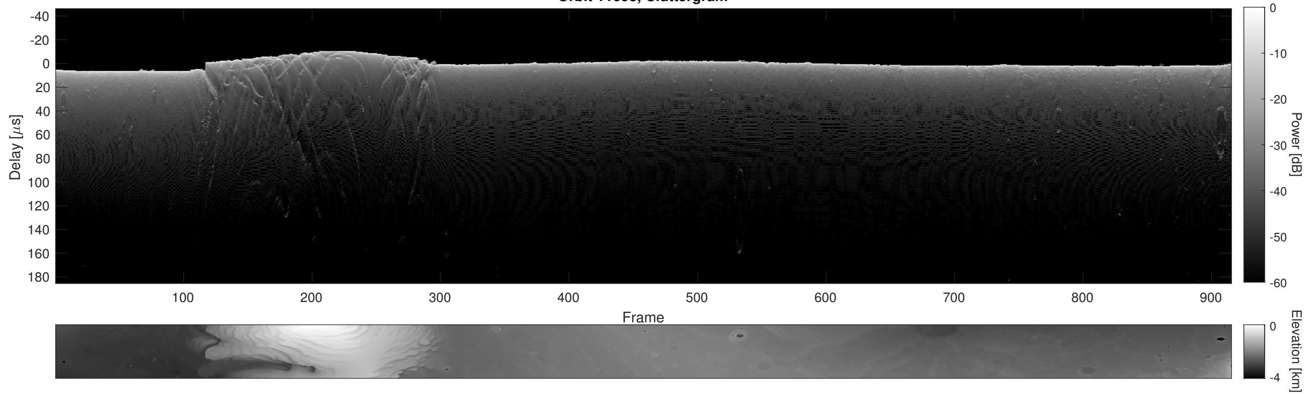
Orbit 11698, Cluttergram
