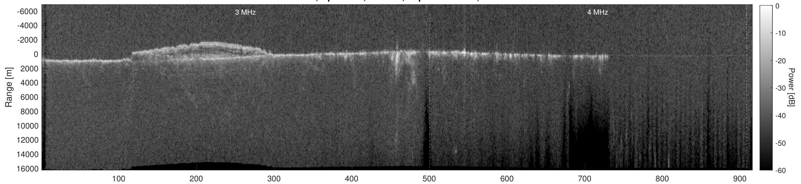
Orbit 11698, Depth-Corrected Cluttergram
