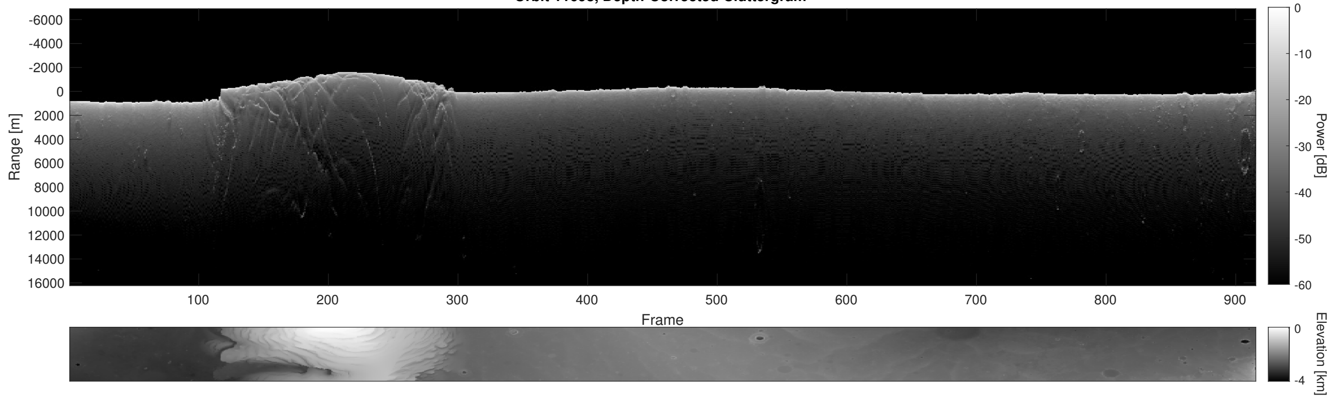
Orbit 11698, Depth-Corrected Cluttergram
