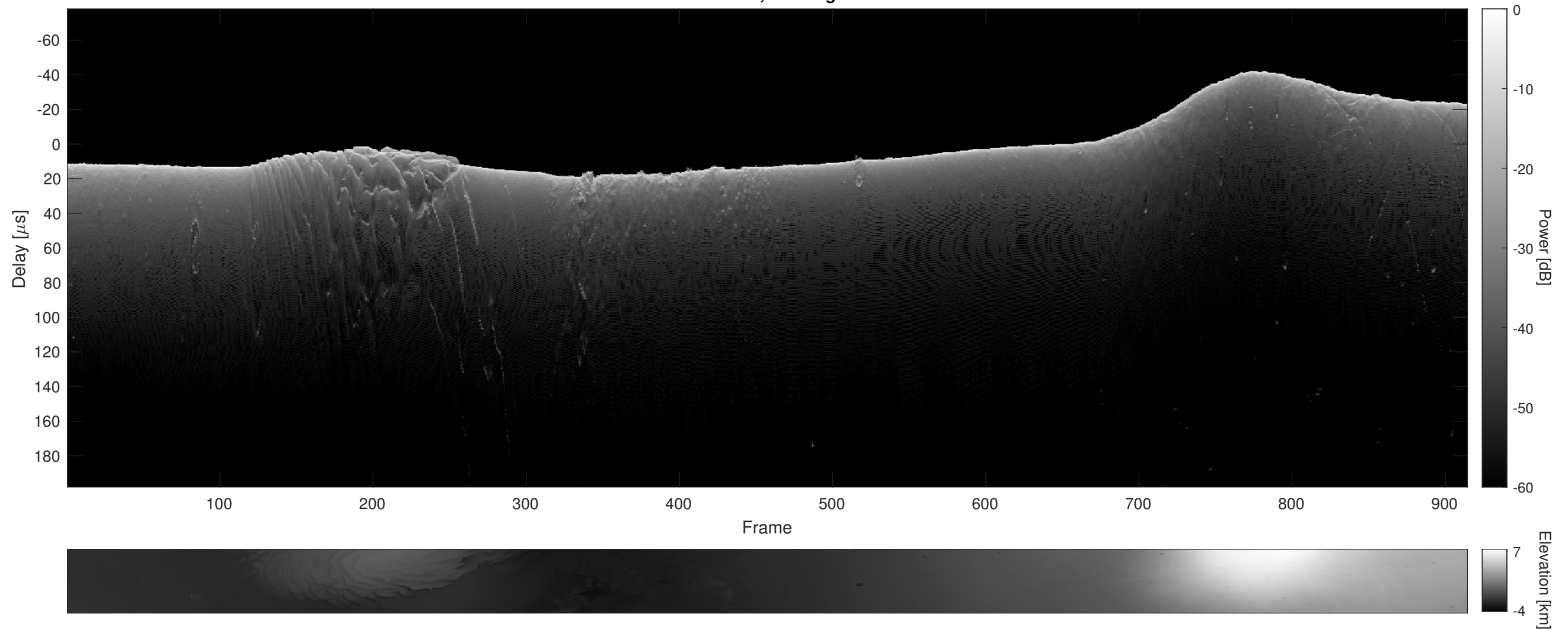
Orbit 11700, Cluttergram
