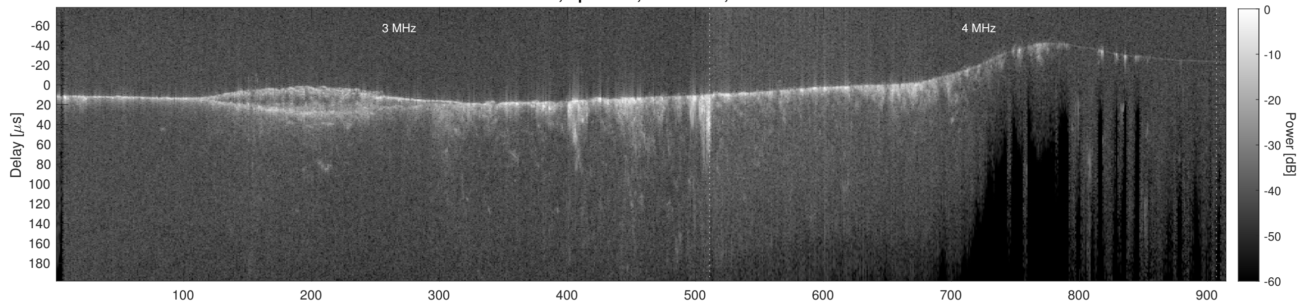
Orbit 11700, Cluttergram
