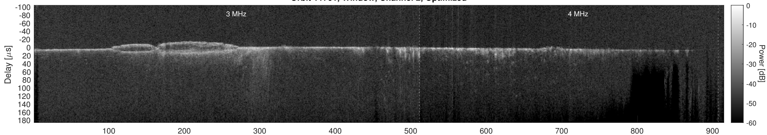
Orbit 11701, Cluttergram
