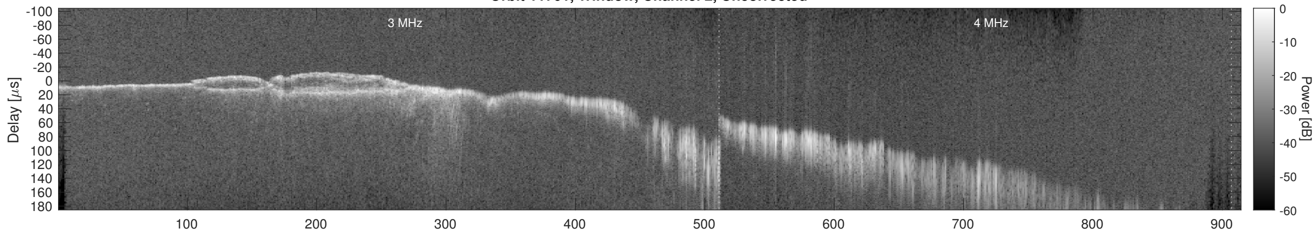
Orbit 11701, Window, Channel 2, Chapman
