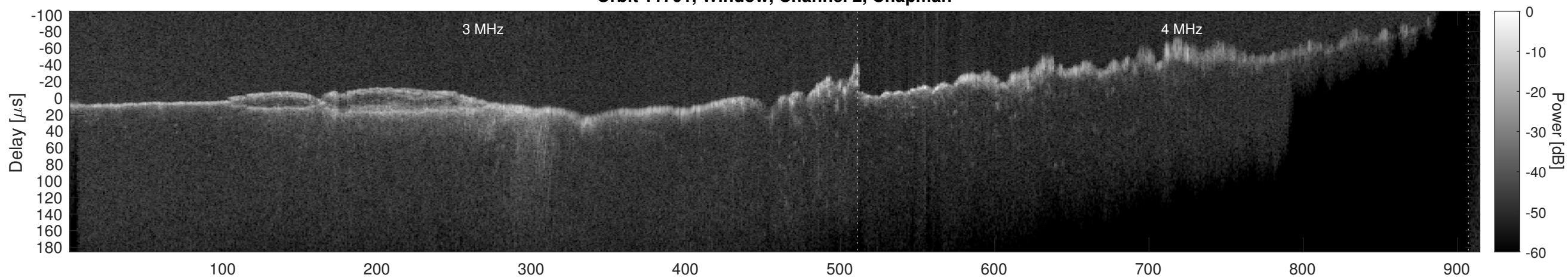
Orbit 11701, Window, Channel 2, Optimized
