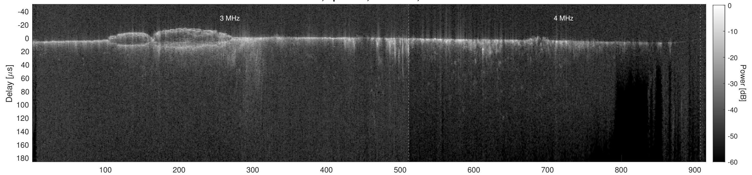
Orbit 11701, Cluttergram
