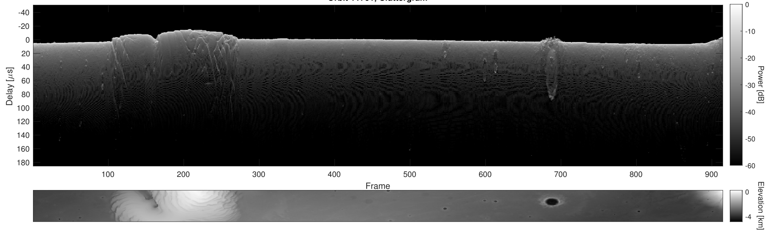
Orbit 11701, Cluttergram
