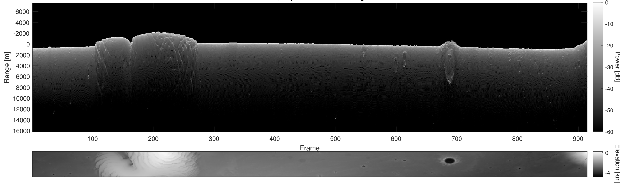
Orbit 11701, Depth-Corrected Cluttergram
