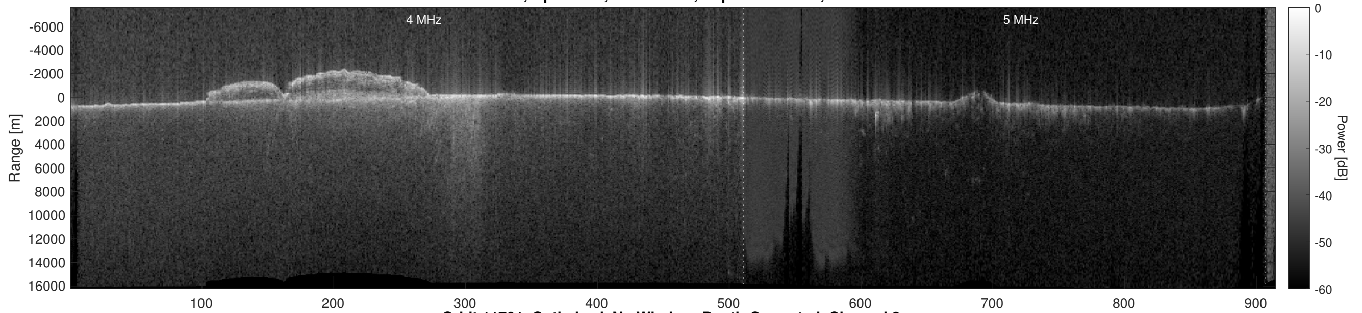
Orbit 11701, Optimized, No Window, Depth-Corrected, Channel 2
