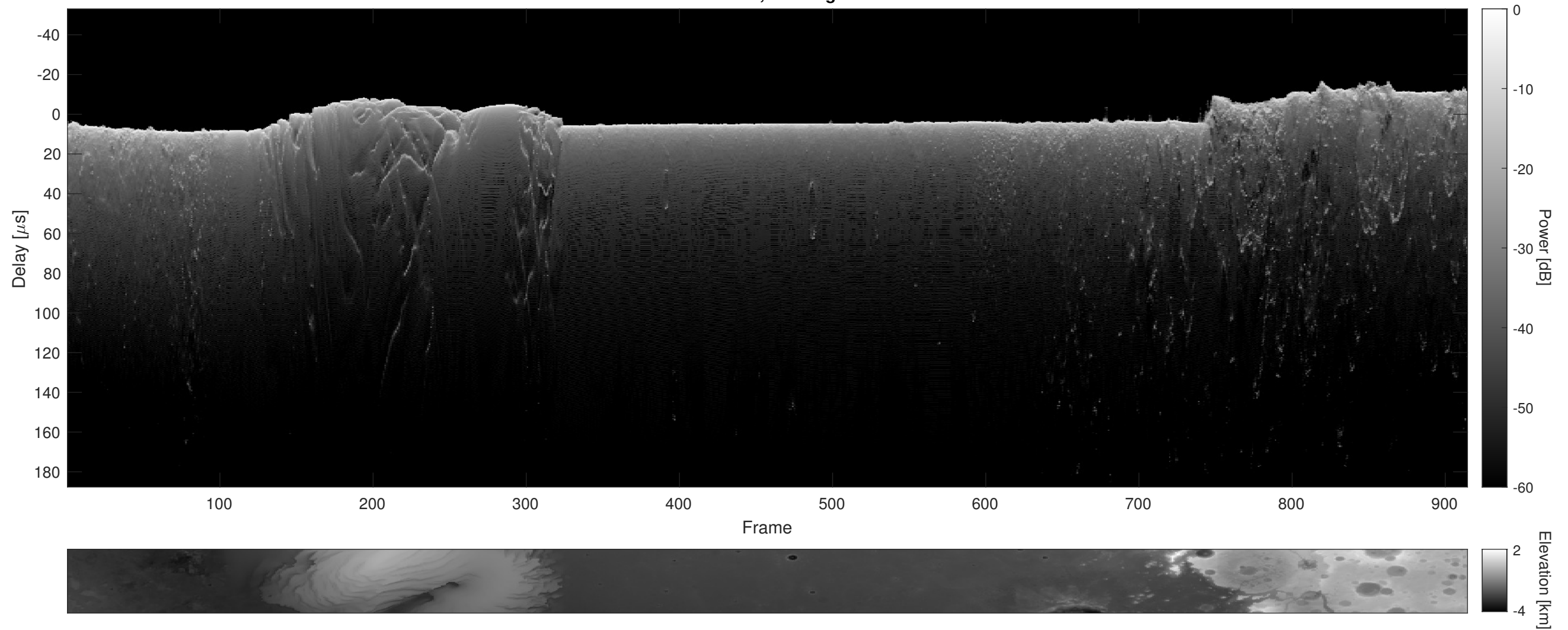
Orbit 11702, Cluttergram
