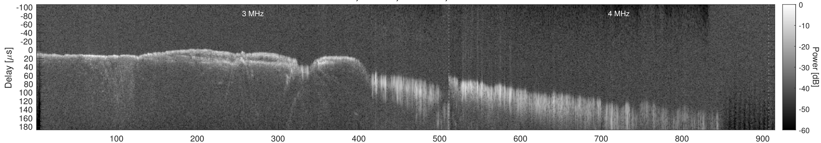
Orbit 11702, Window, Channel 2, Chapman
