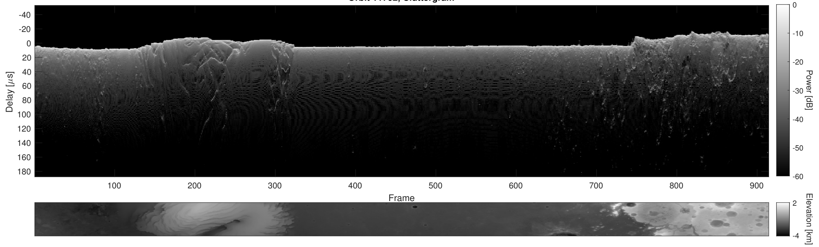
Orbit 11702, Cluttergram
