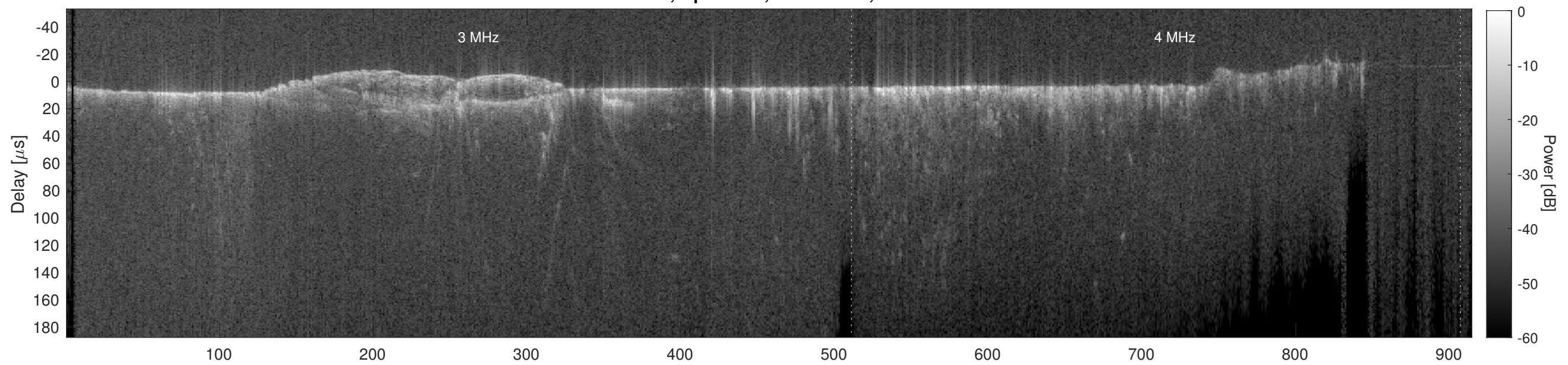
Orbit 11702, Cluttergram
