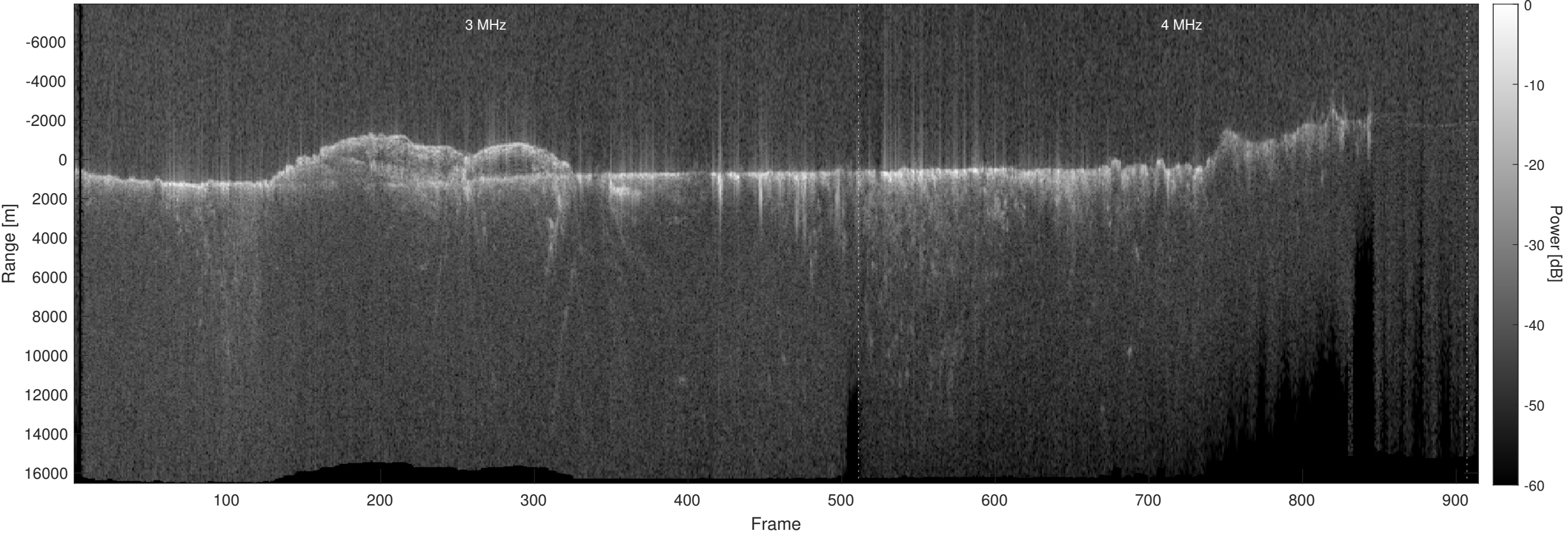
Orbit 11702, Optimized, No Window, Depth-Corrected, Channel 2
