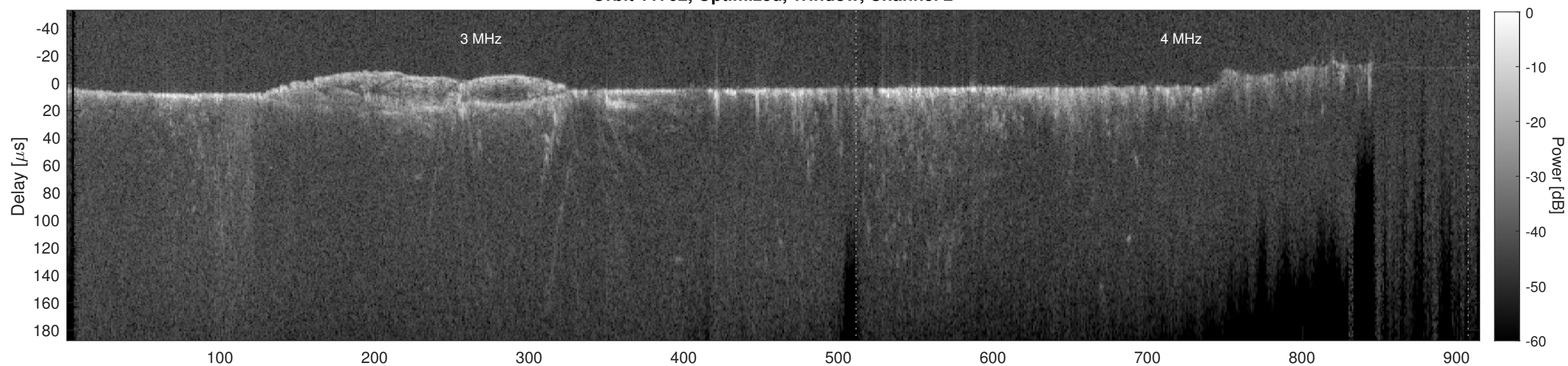
Orbit 11702, Cluttergram
