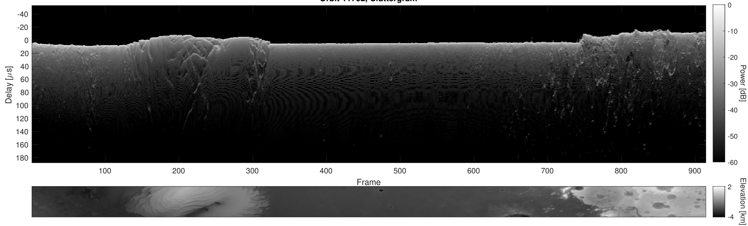
Orbit 11702, Cluttergram
