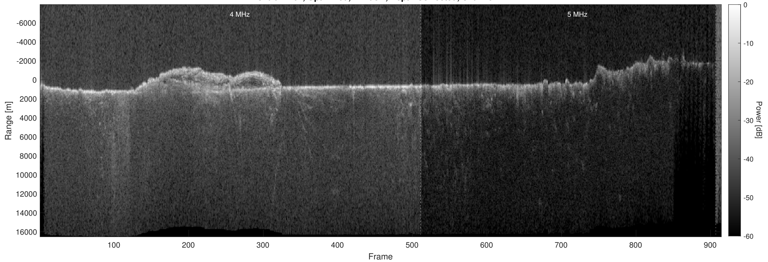
Orbit 11702, Optimized, Window, Depth-Corrected, Channel 2
