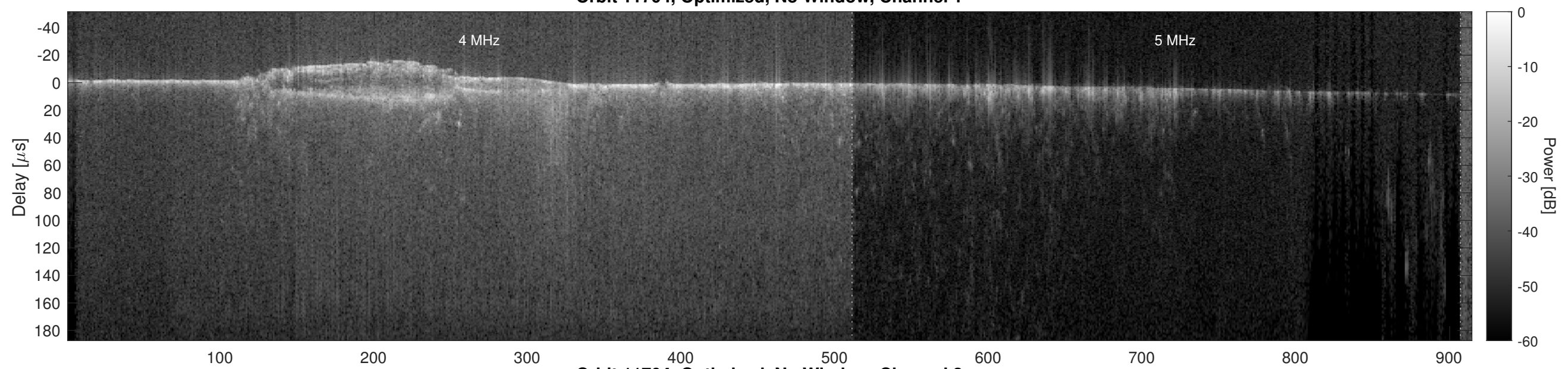
Orbit 11704, Optimized, No Window, Channel 2
