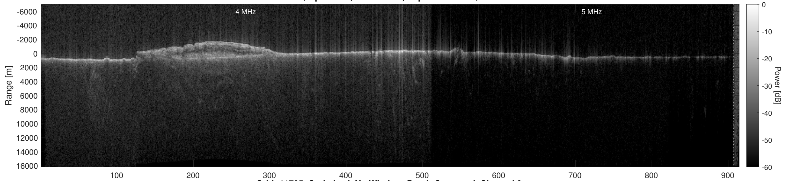
Orbit 11705, Optimized, No Window, Depth-Corrected, Channel 2
