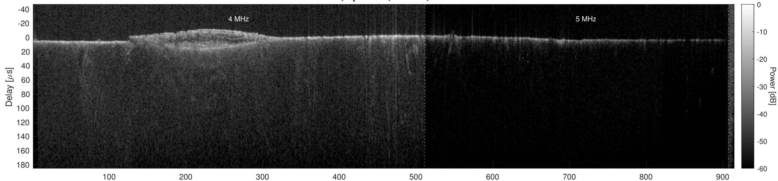
Orbit 11705, Optimized, Window, Channel 2
