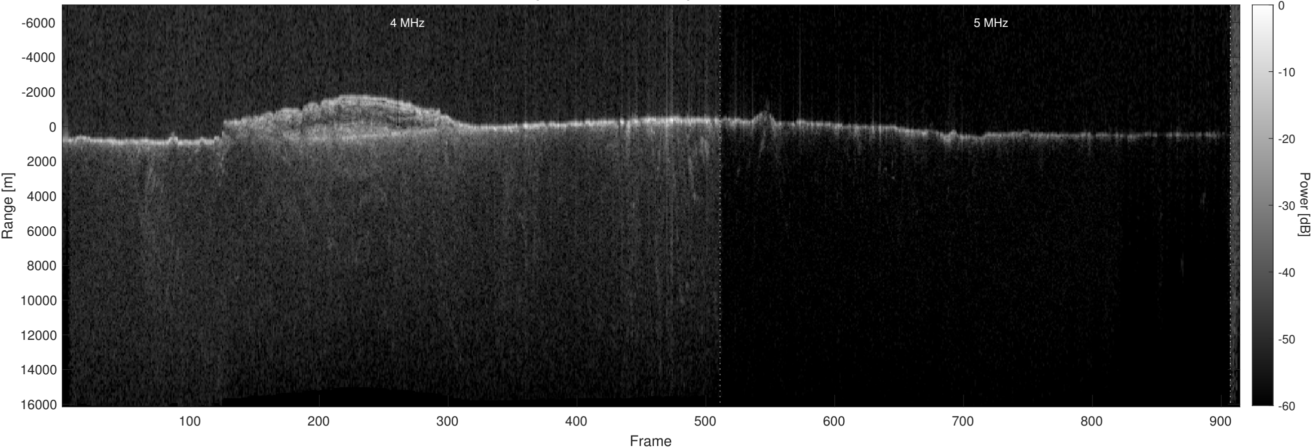
Orbit 11705, Optimized, Window, Depth-Corrected, Channel 2
