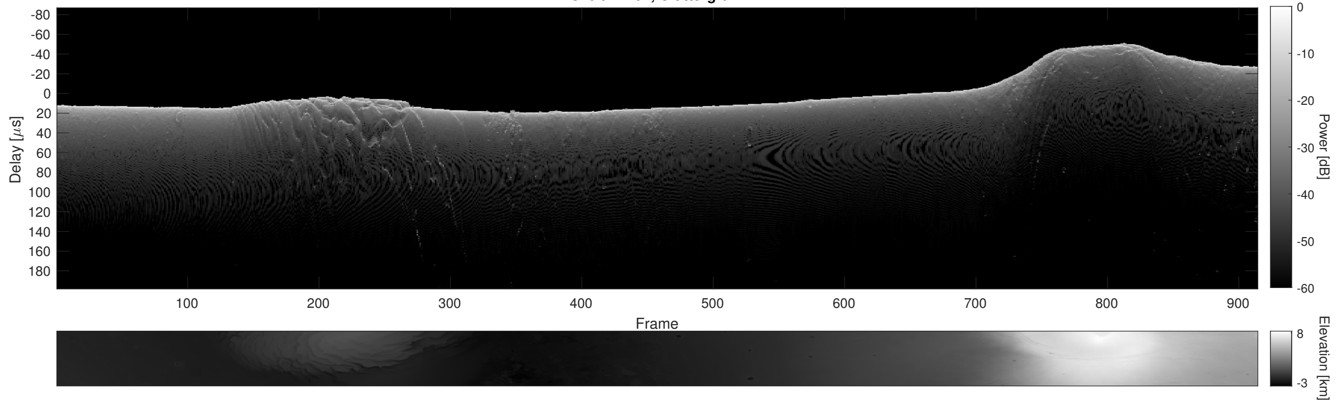
Orbit 11707, Cluttergram
