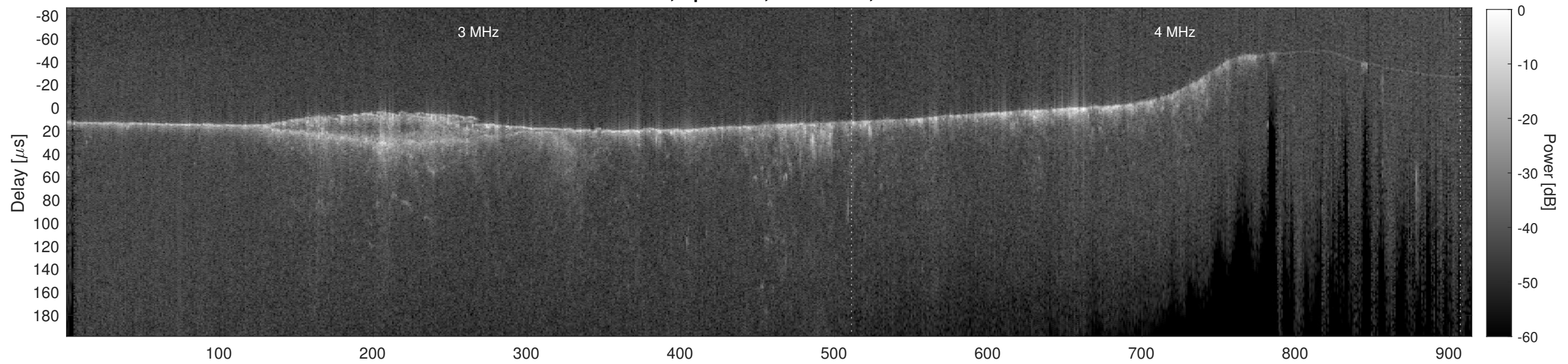
Orbit 11707, Cluttergram
