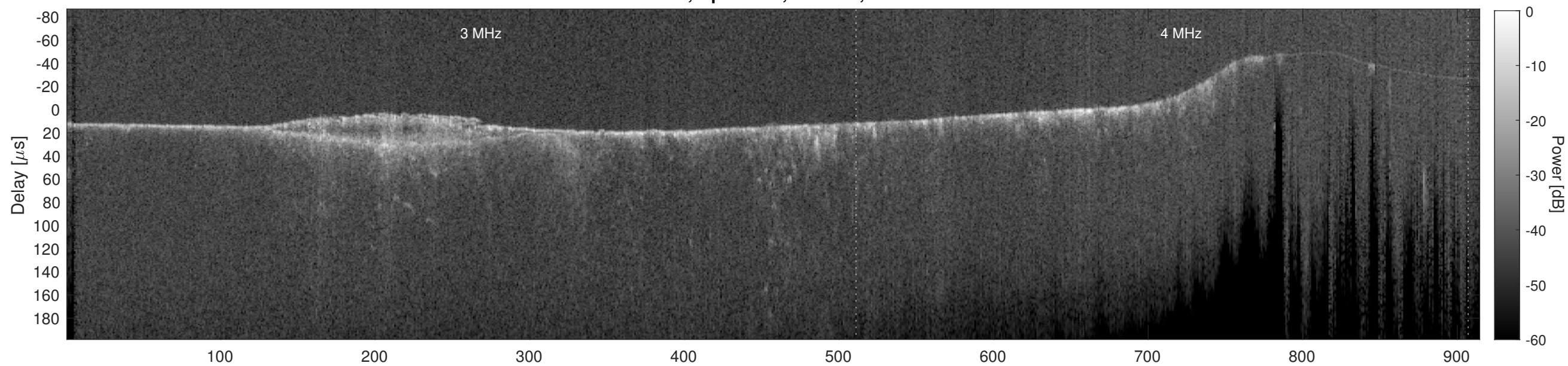
Orbit 11707, Cluttergram
