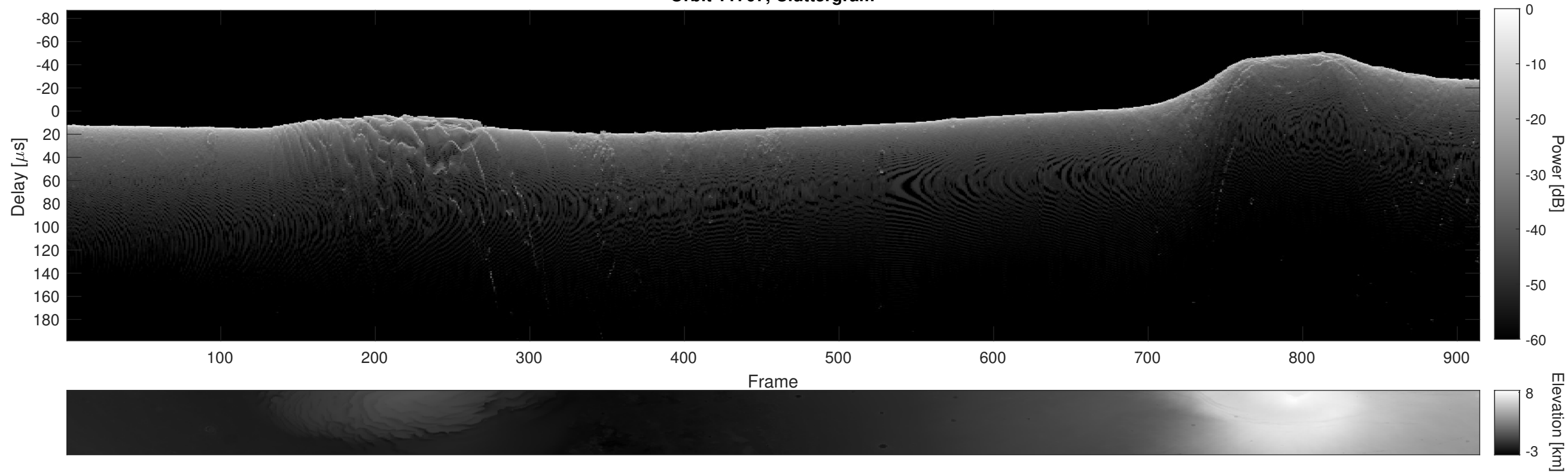
Orbit 11707, Cluttergram
