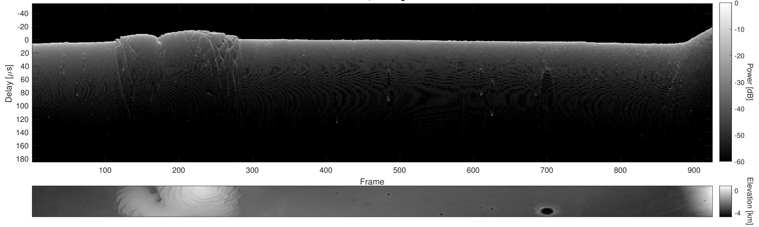
Orbit 11708, Cluttergram
