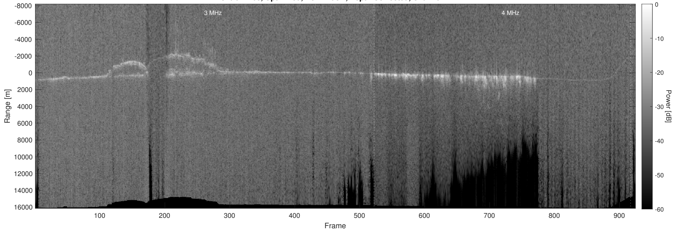
Orbit 11708, Optimized, No Window, Depth-Corrected, Channel 2
