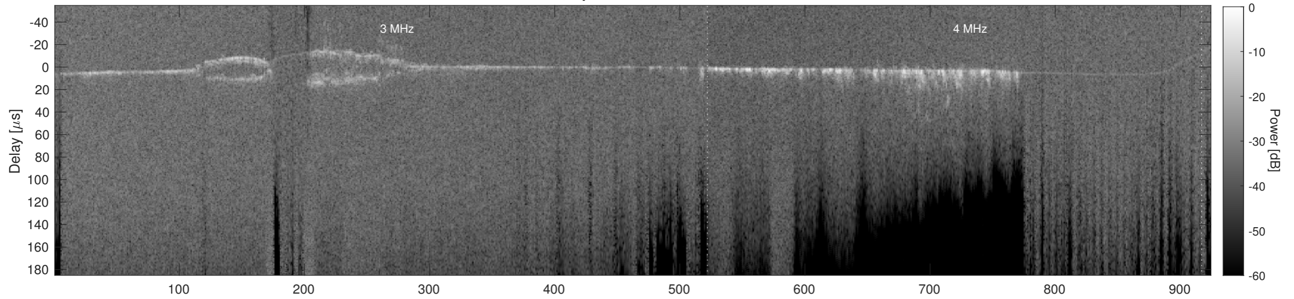
Orbit 11708, Cluttergram
