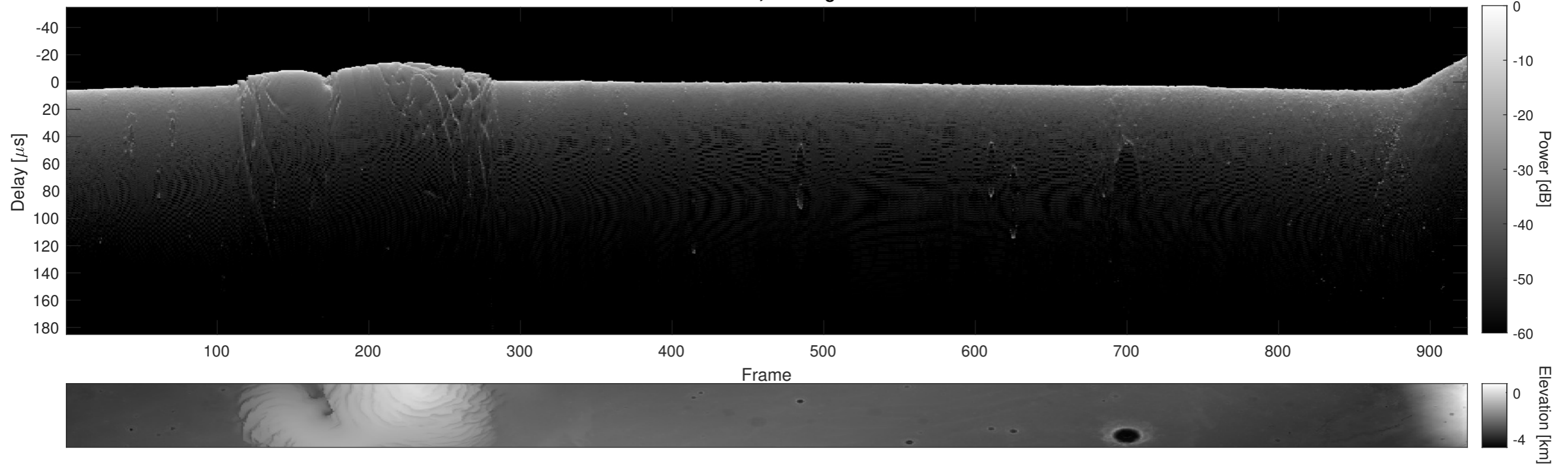
Orbit 11708, Cluttergram
