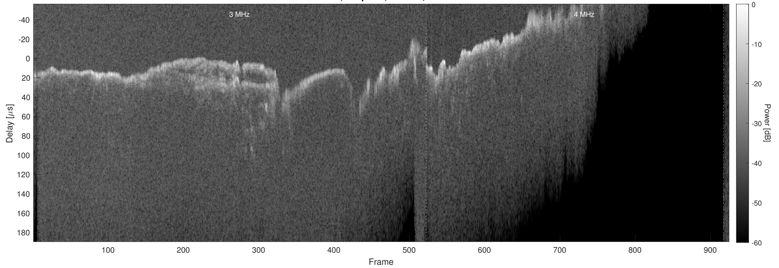
Orbit 11709, Chapman, Window, Channel 2
