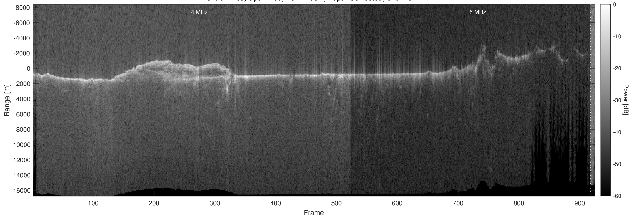
Orbit 11709, Optimized, No Window, Depth-Corrected, Channel 2
