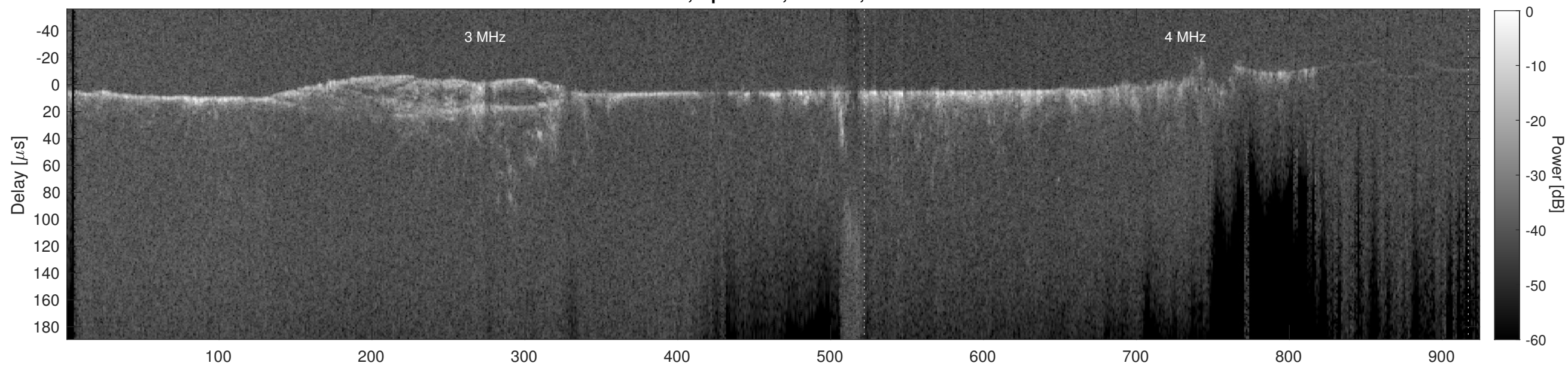
Orbit 11709, Cluttergram
