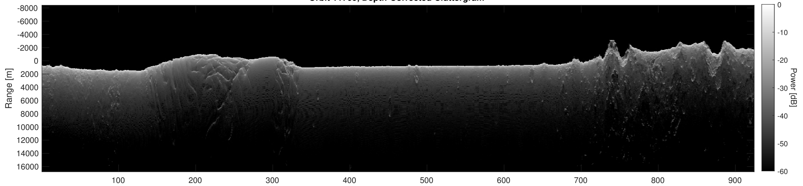
Orbit 11709, Depth-Corrected Cluttergram
