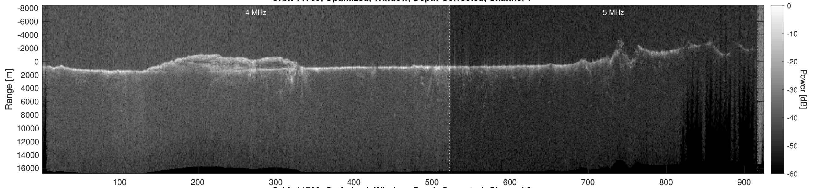
Orbit 11709, Optimized, Window, Depth-Corrected, Channel 2
