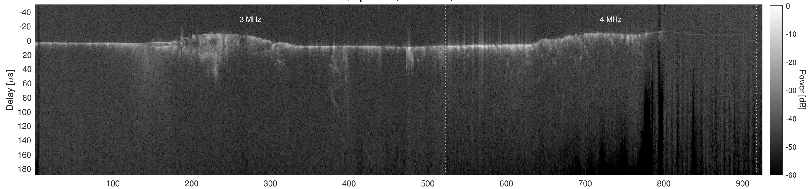
Orbit 11710, Cluttergram
