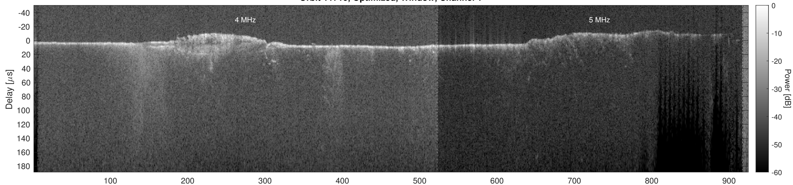
Orbit 11710, Optimized, Window, Channel 2
