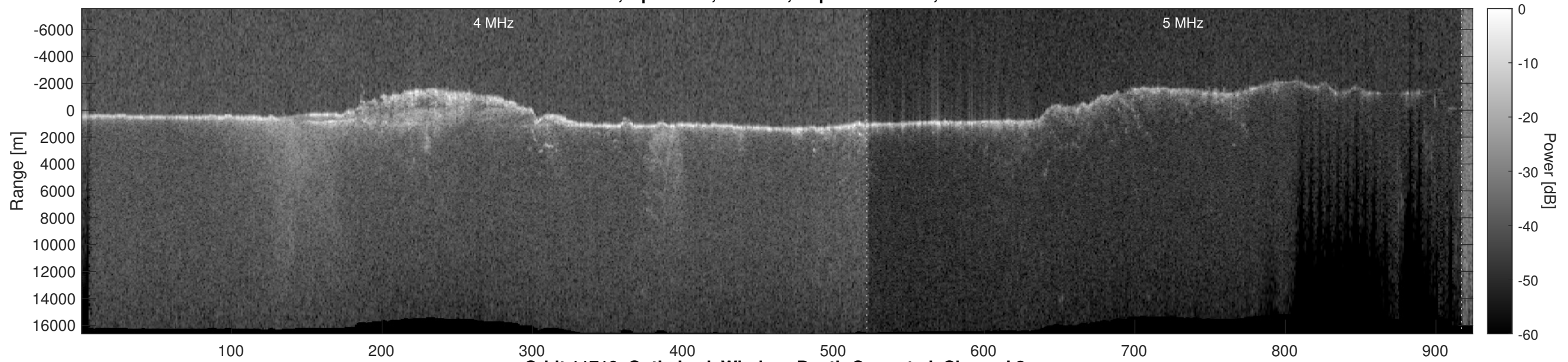
Orbit 11710, Optimized, Window, Depth-Corrected, Channel 2
