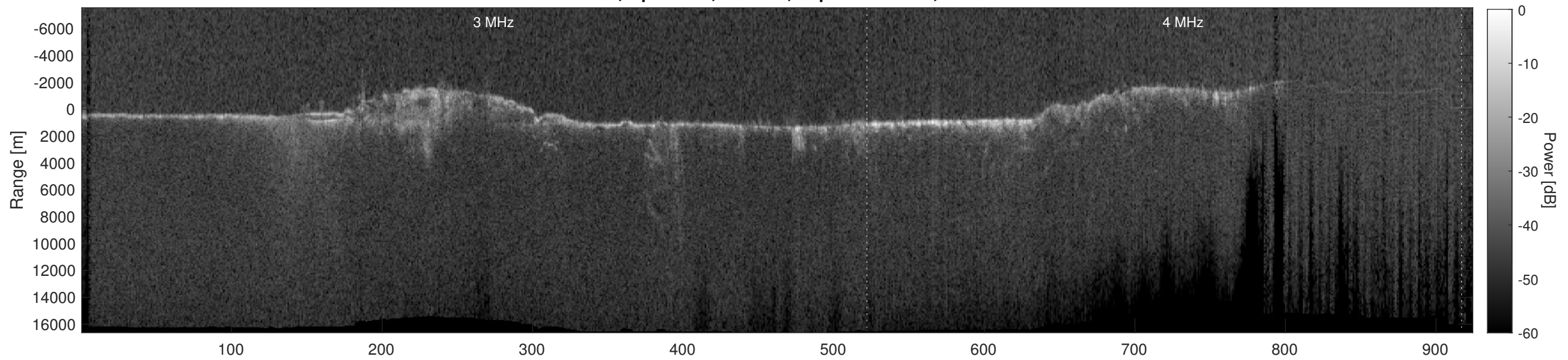
Orbit 11710, Depth-Corrected Cluttergram
