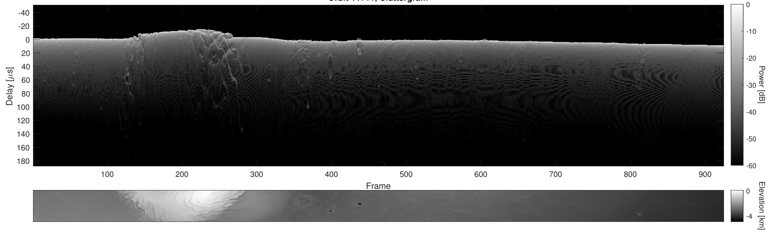
Orbit 11711, Cluttergram
