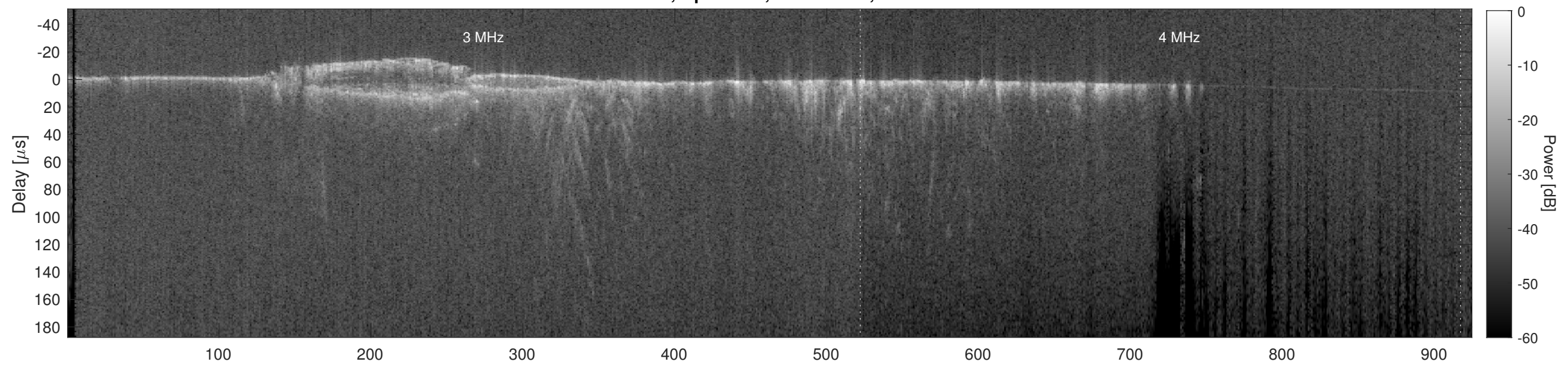
Orbit 11711, Cluttergram
