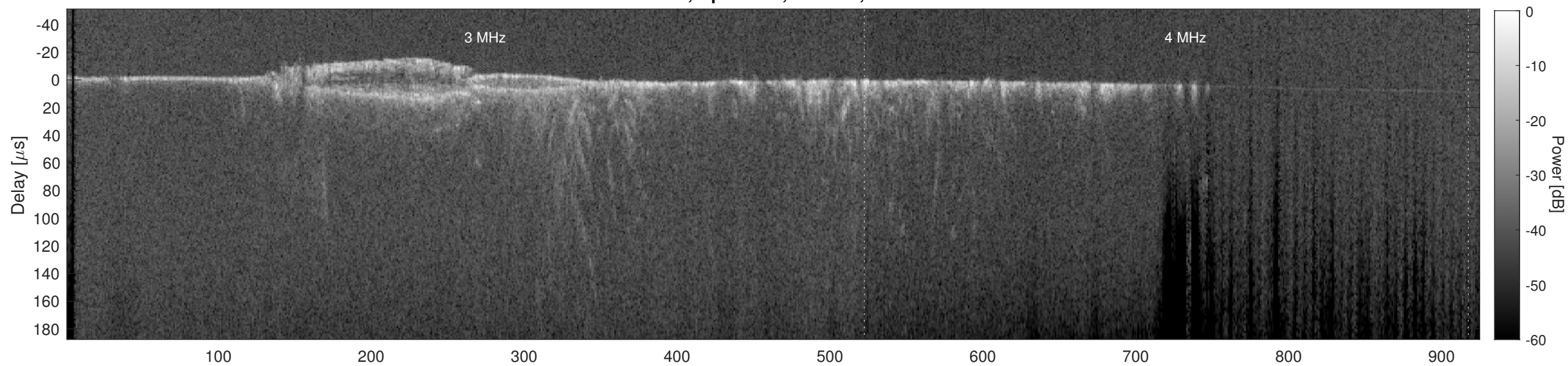
Orbit 11711, Cluttergram
