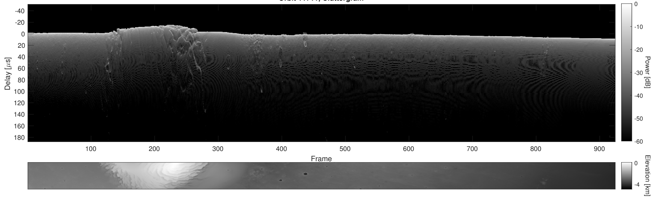
Orbit 11711, Cluttergram
