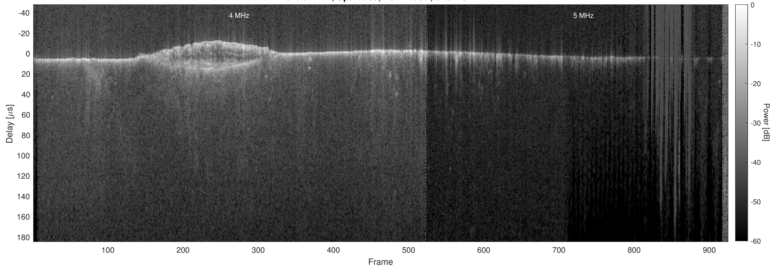
Orbit 11712, Optimized, No Window, Channel 2
