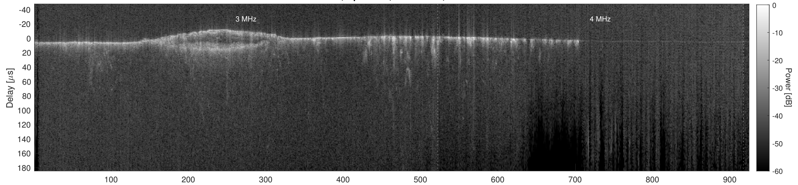
Orbit 11712, Cluttergram
