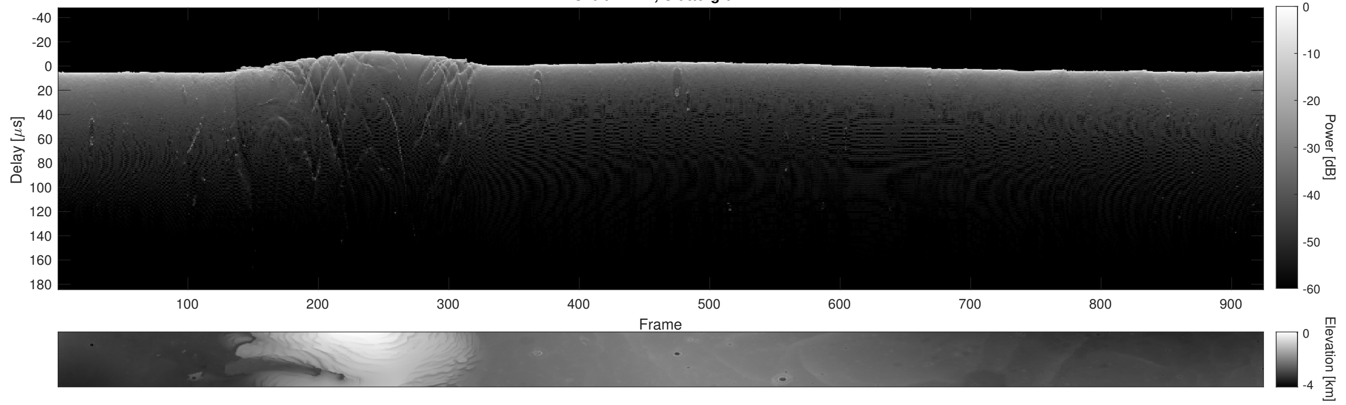
Orbit 11712, Cluttergram
