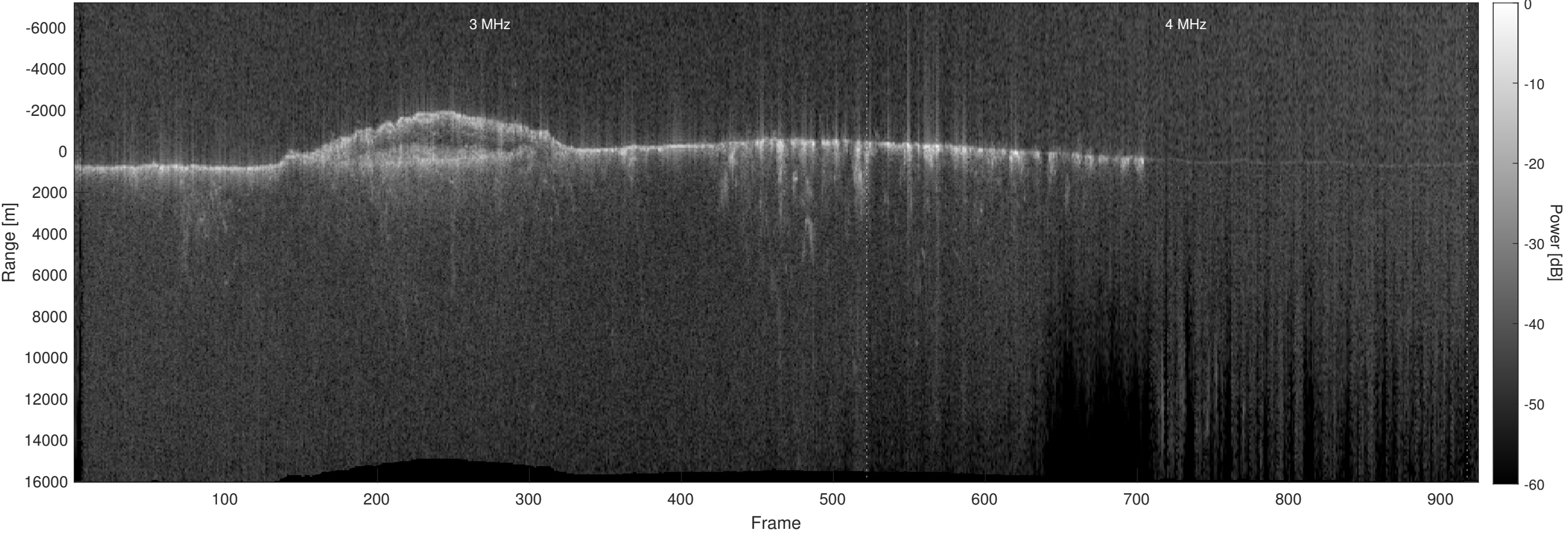
Orbit 11712, Optimized, No Window, Depth-Corrected, Channel 2
