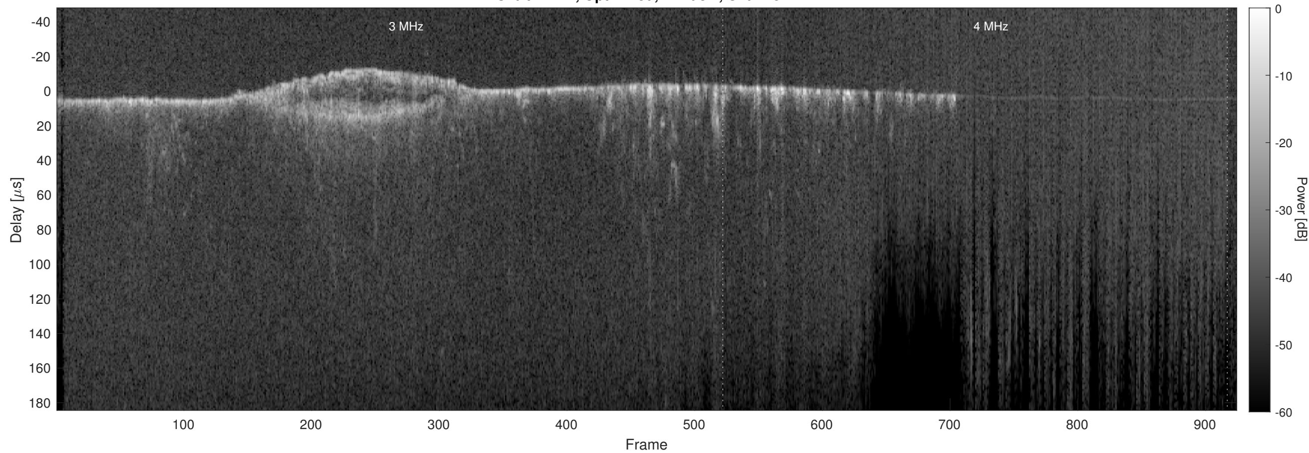
Orbit 11712, Optimized, Window, Channel 2
