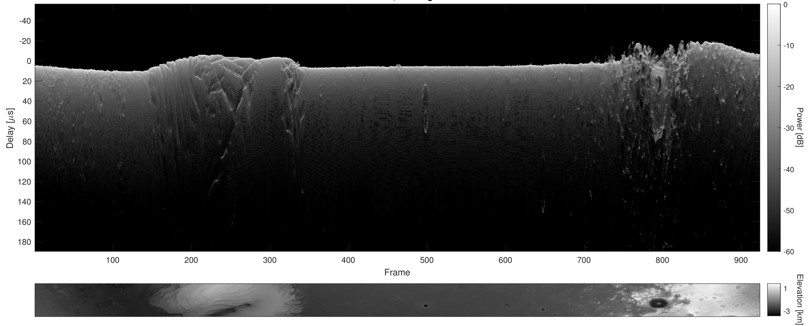
Orbit 11716, Cluttergram
