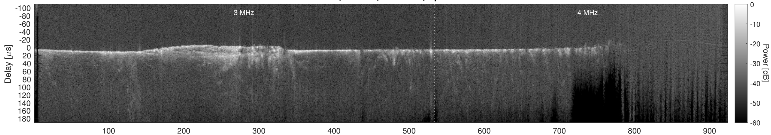
Orbit 11716, Cluttergram
