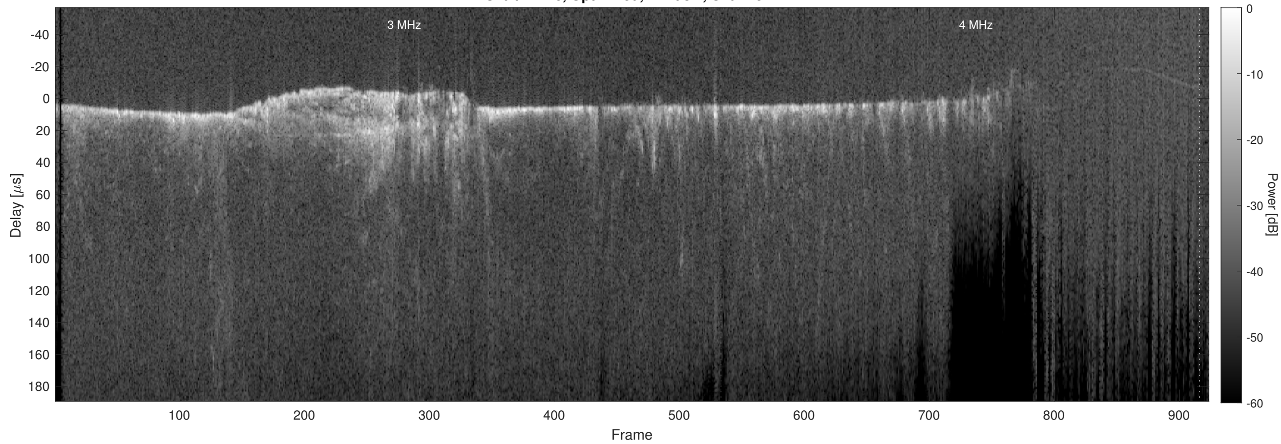
Orbit 11716, Optimized, Window, Channel 2
