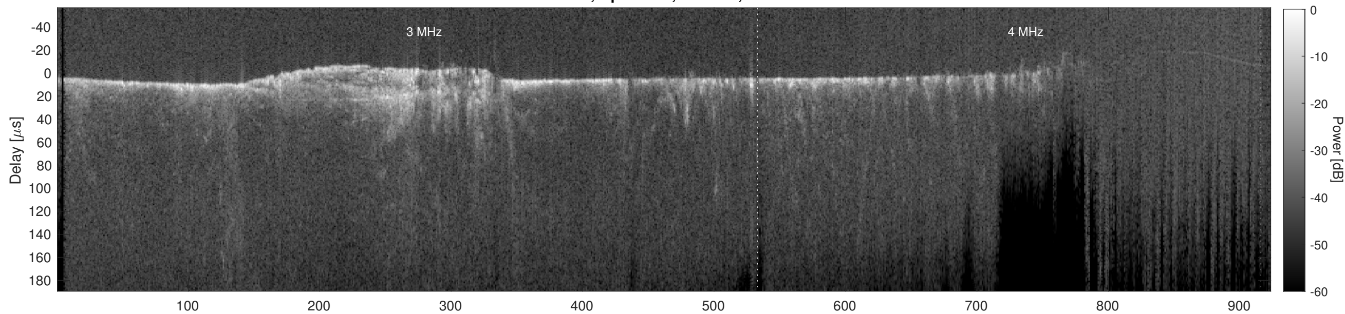
Orbit 11716, Cluttergram
