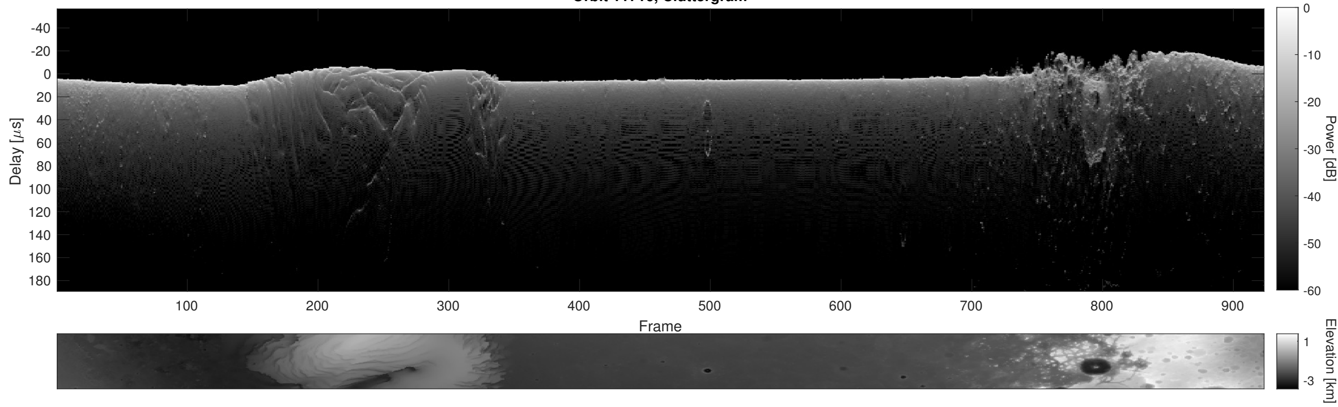
Orbit 11716, Cluttergram
