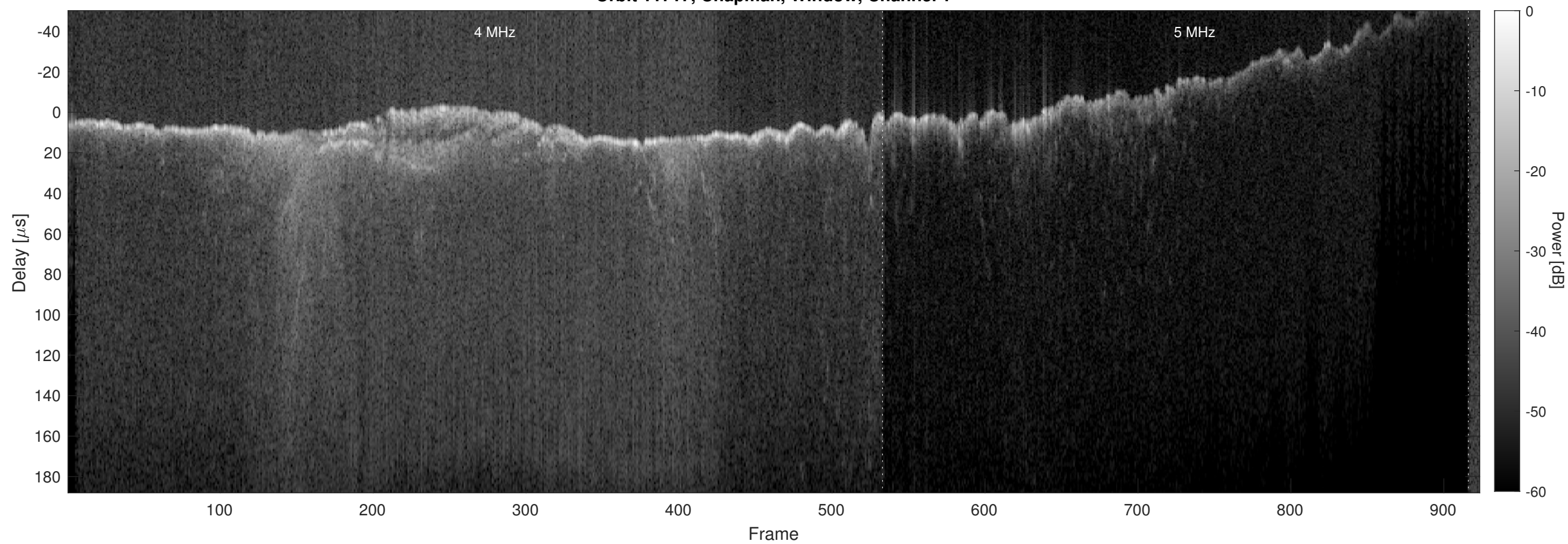
Orbit 11717, Chapman, Window, Channel 2
