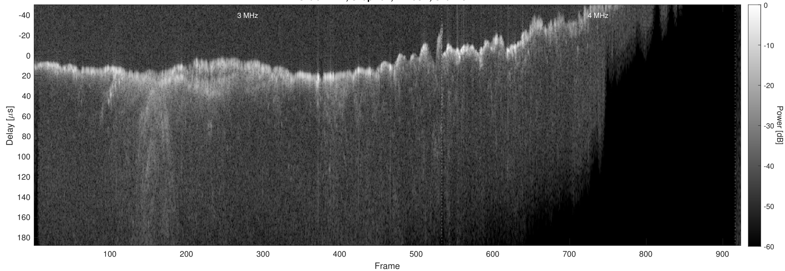
Orbit 11717, Chapman, Window, Channel 2
