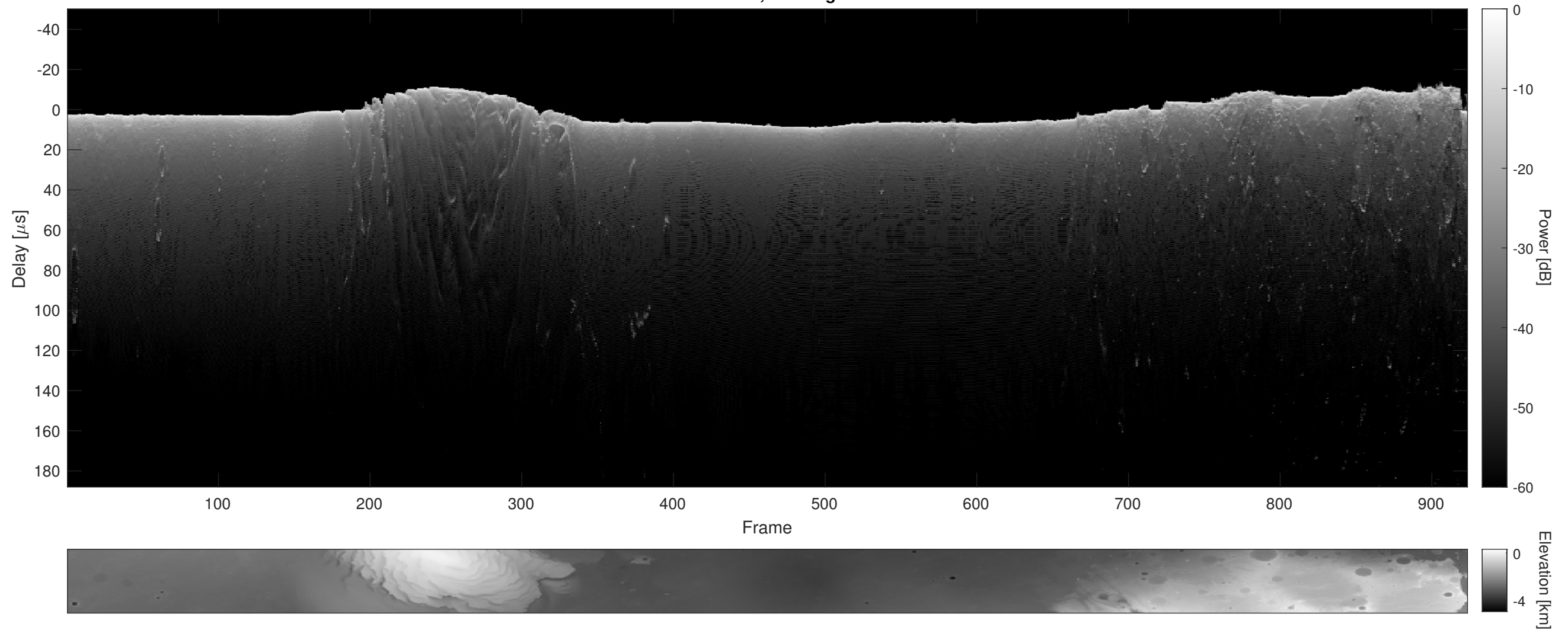
Orbit 11717, Cluttergram
