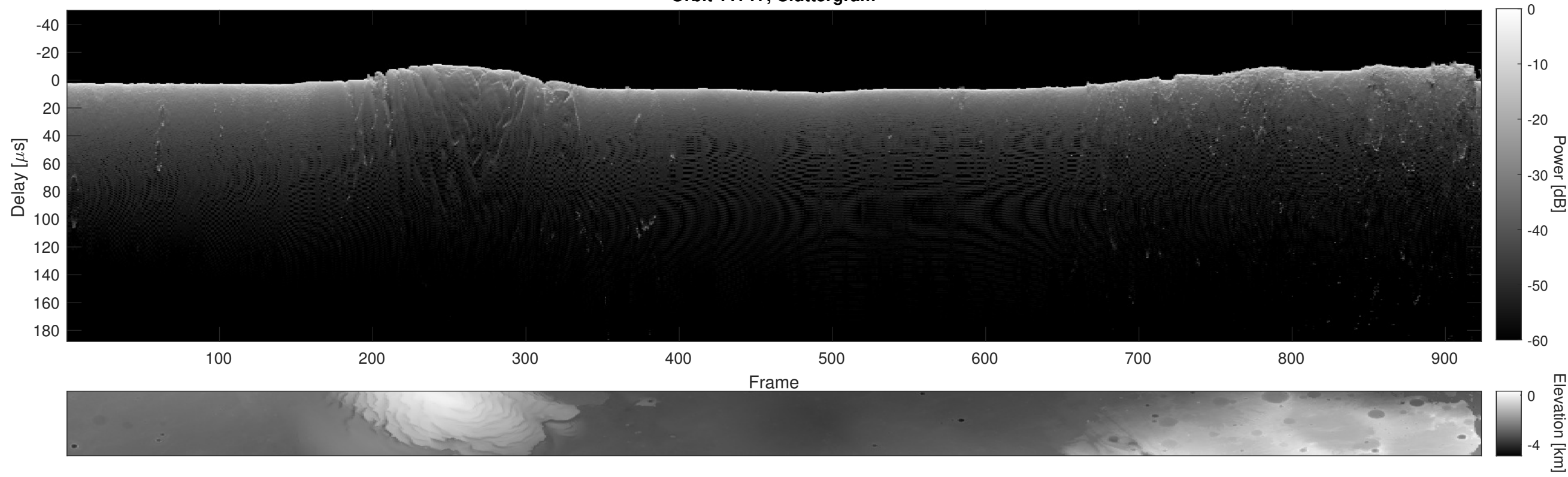
Orbit 11717, Cluttergram
