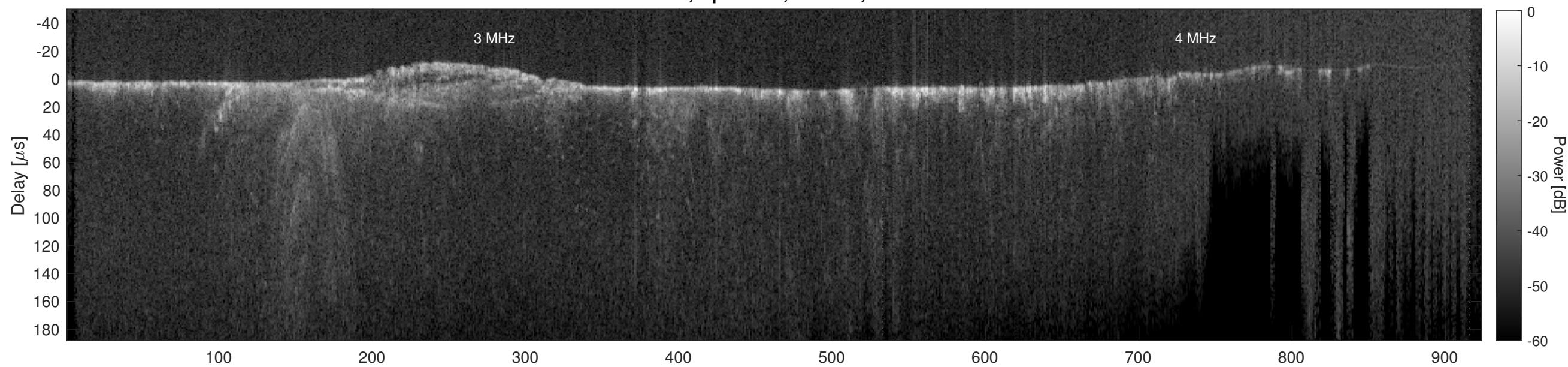
Orbit 11717, Cluttergram
