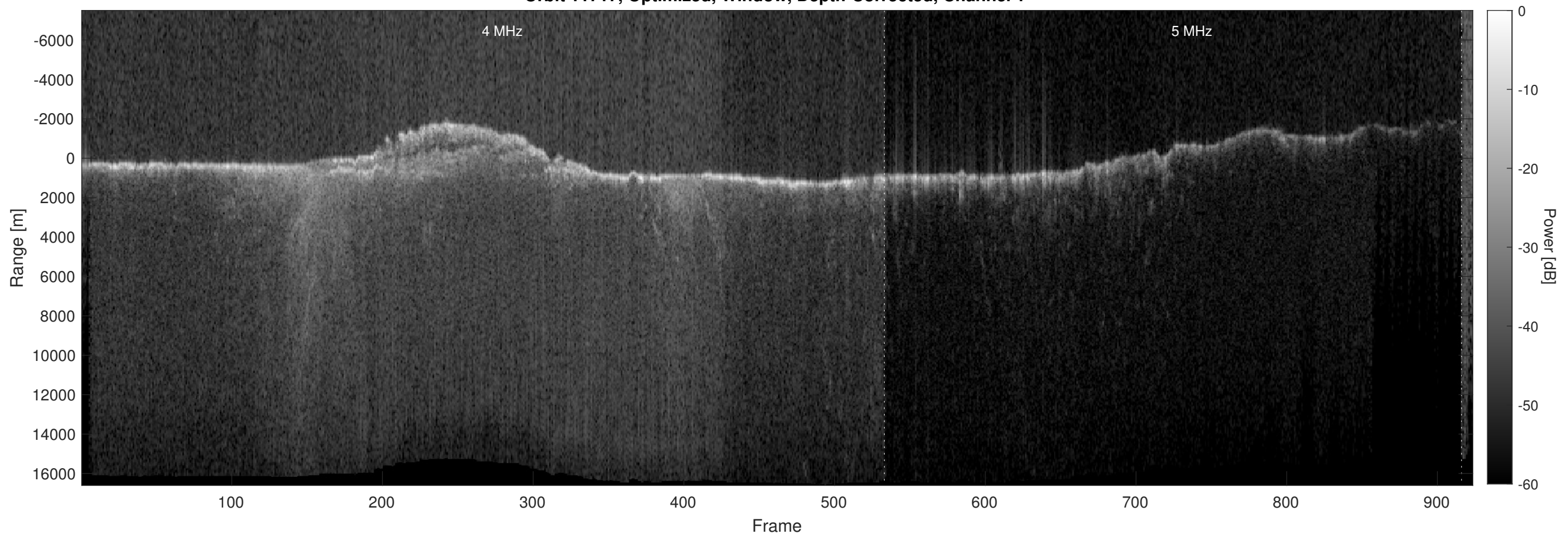
Orbit 11717, Optimized, Window, Depth-Corrected, Channel 2
